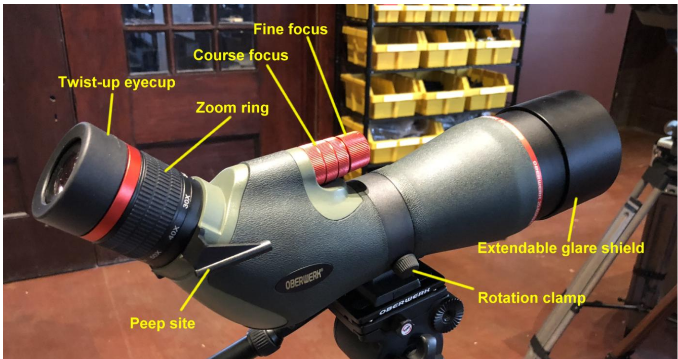
Oberwerk 20-60x82 Sport ED components and controls
